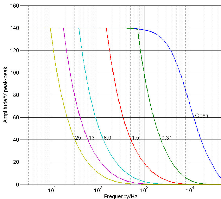
E-610: Operating limits (open loop) with various piezo loads, capacitance values in \mu F
