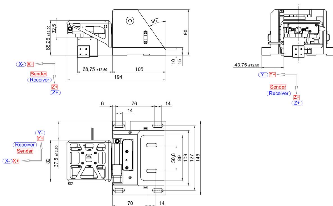
F-712.MA2, dimensions in mm
