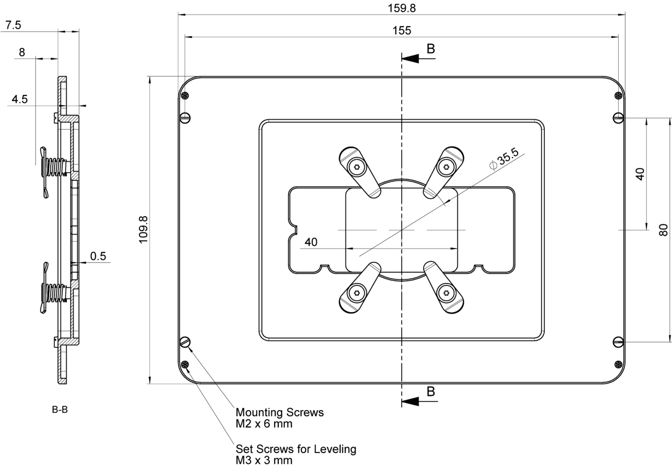
P-736.PDN, dimensions in mm
